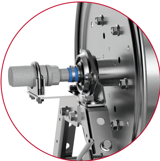
Close-up of CPVC swivel, clamp and mounting bracket.
